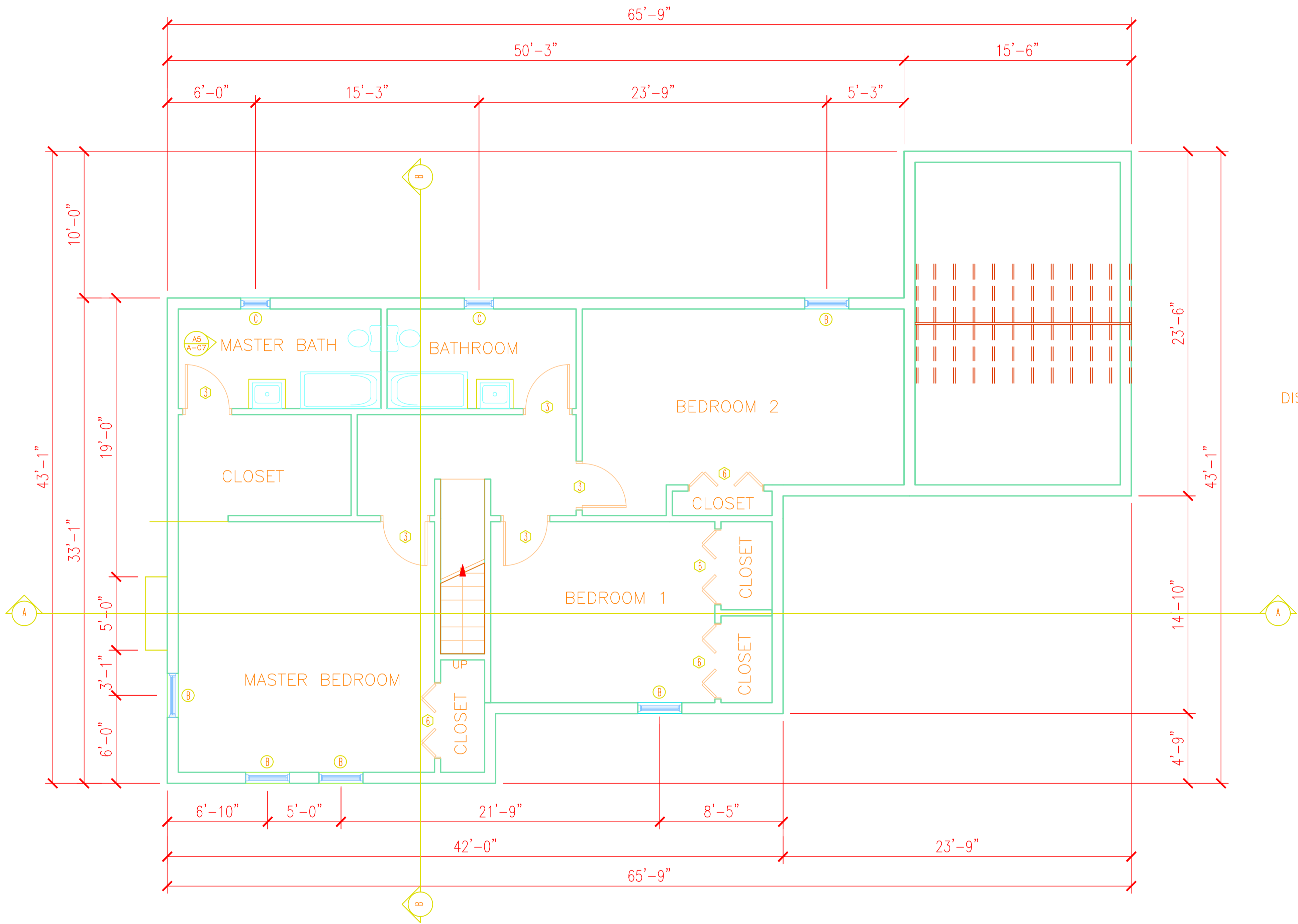
A 005 SECOND FLOOR PLAN SCALE 3/16" = 1'-0"
