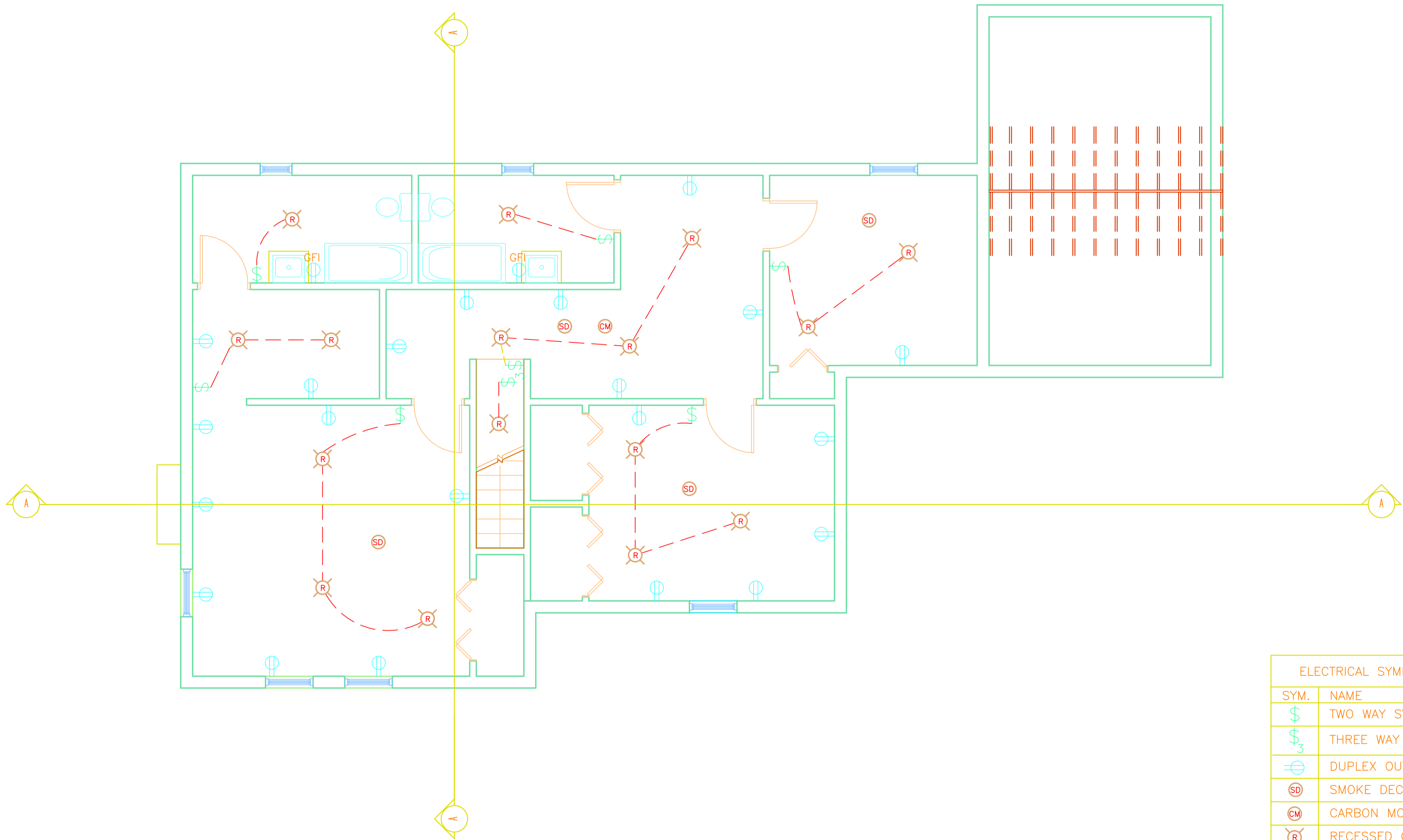
A 016 SECOND FLOOR ELECTRICAL PLAN N ↑ SCALE 3/16"=1'-0"
