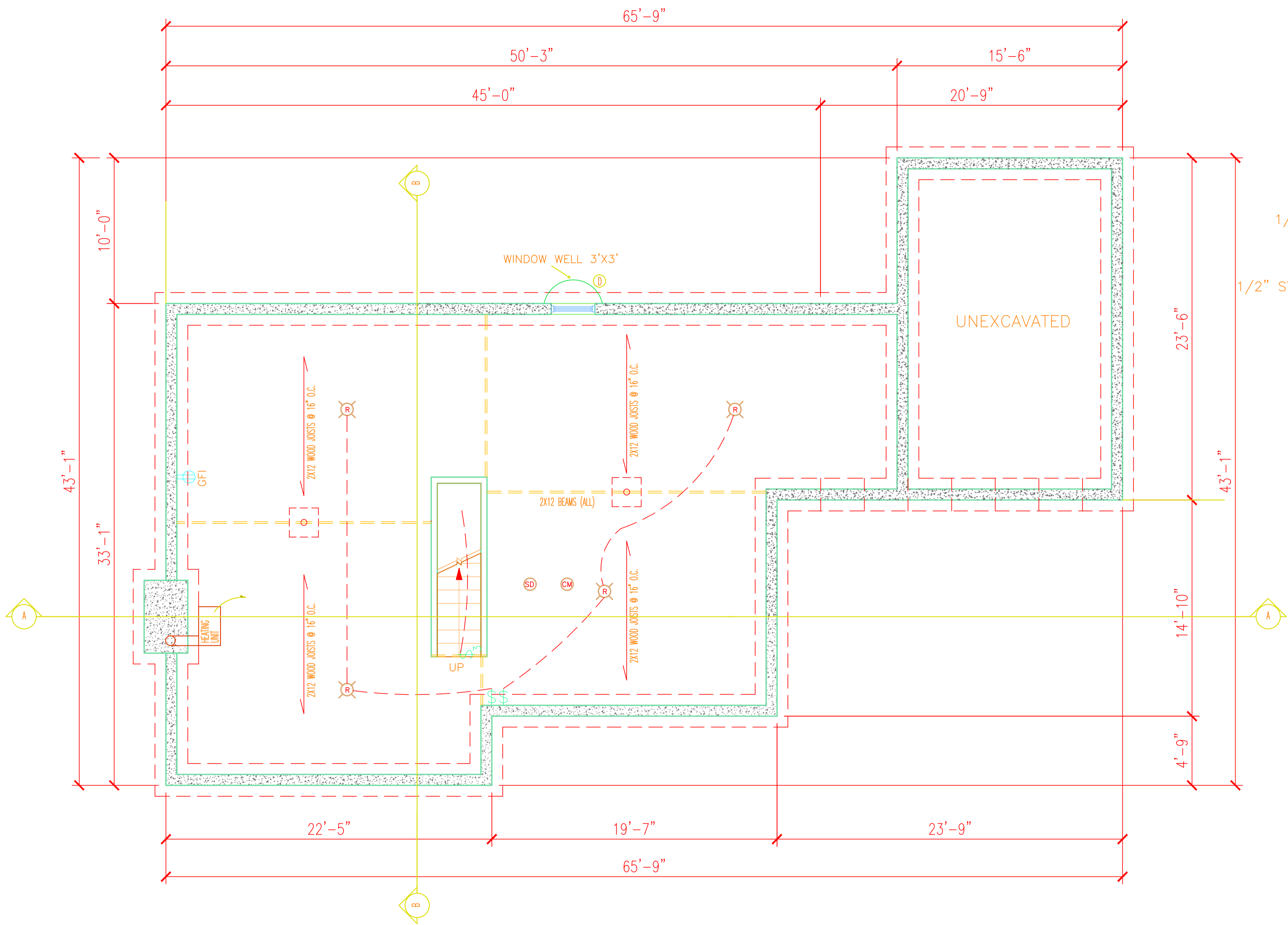
A 003 FOUNDATION FLOOR PLAN SCALE 3/16"=1'-0"
