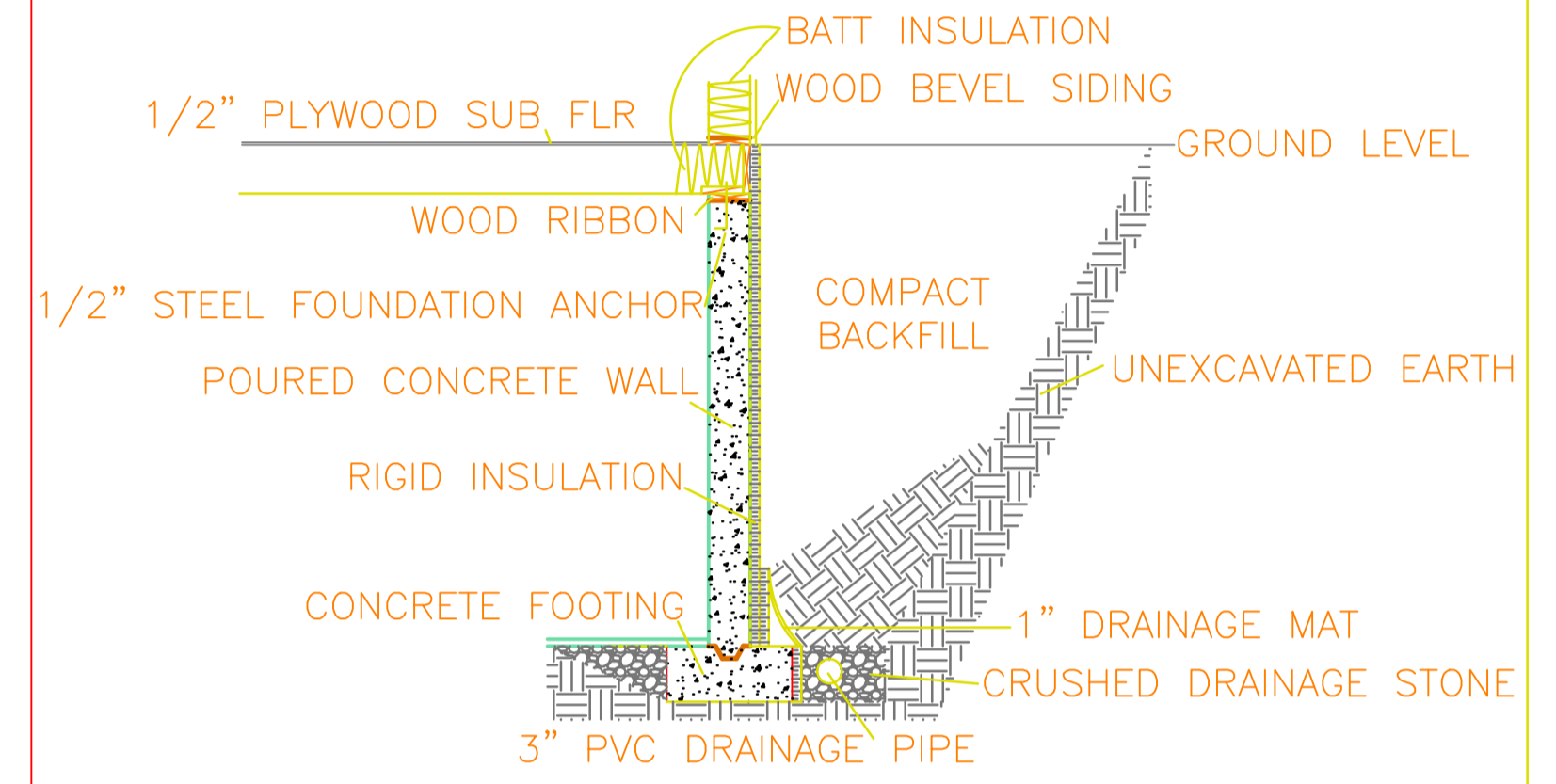
A1 FOUNDATION AND EXTERIOR WALL DETAIL
