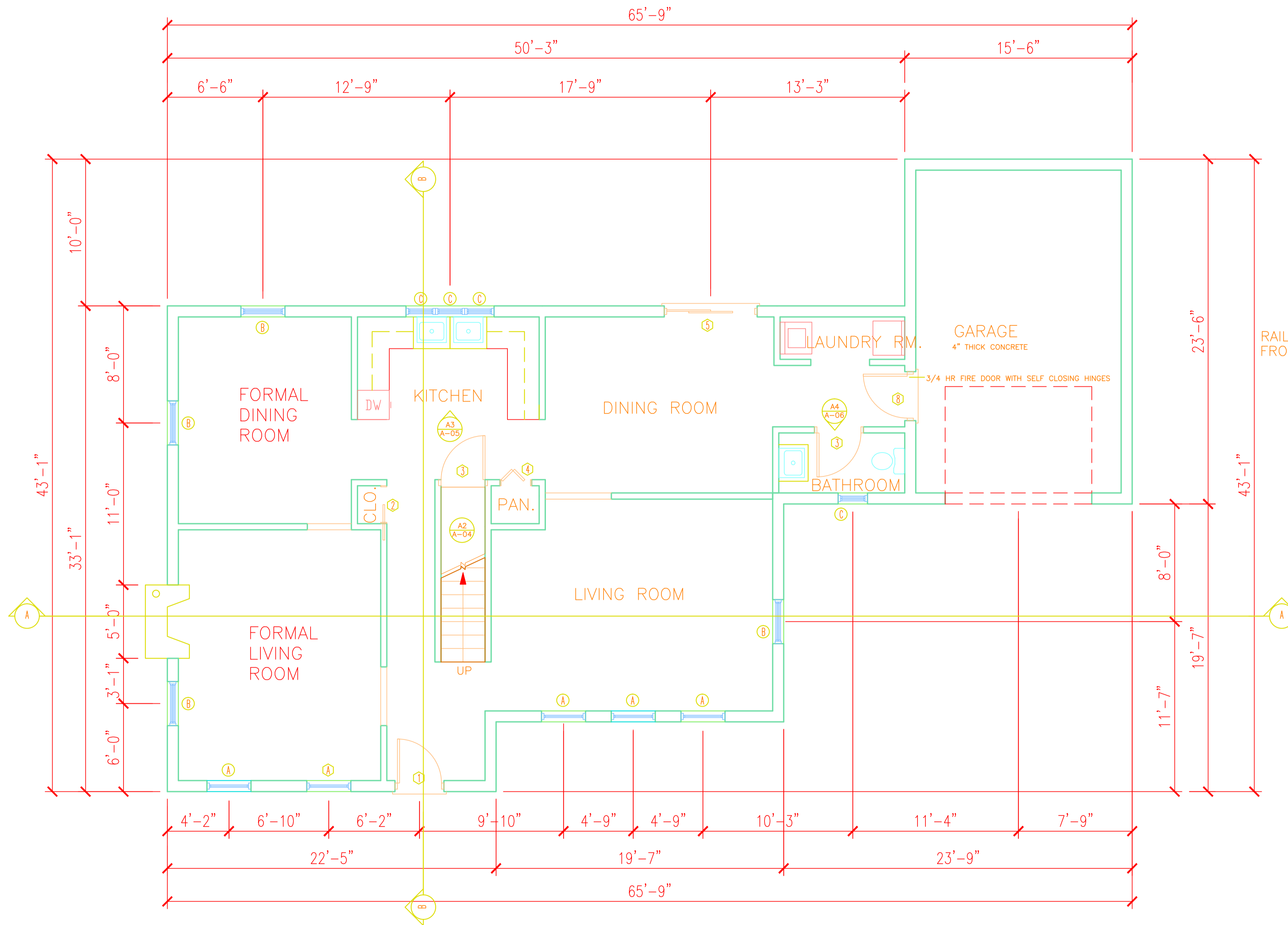
A 004 FIRST FLOOR PLAN SCALE 3/16" = 1'-0"
