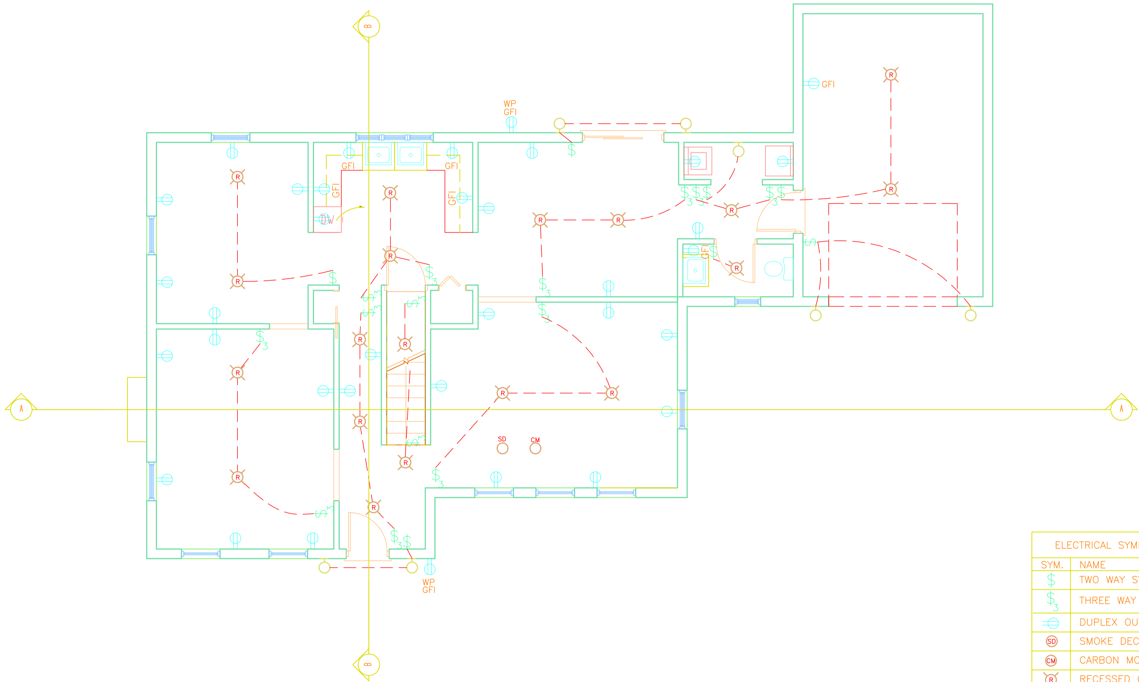
A 015 FIRST FLOOR ELECTRICAL PLAN N ↑ SCALE 3/16" = 1'-0"
