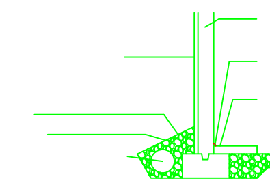
WALL DETAIL Scale: 1/4"=1.0'
