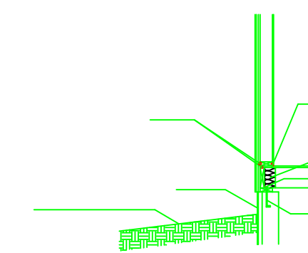
WALL DETAIL Scale: 1/4"=1.0'
