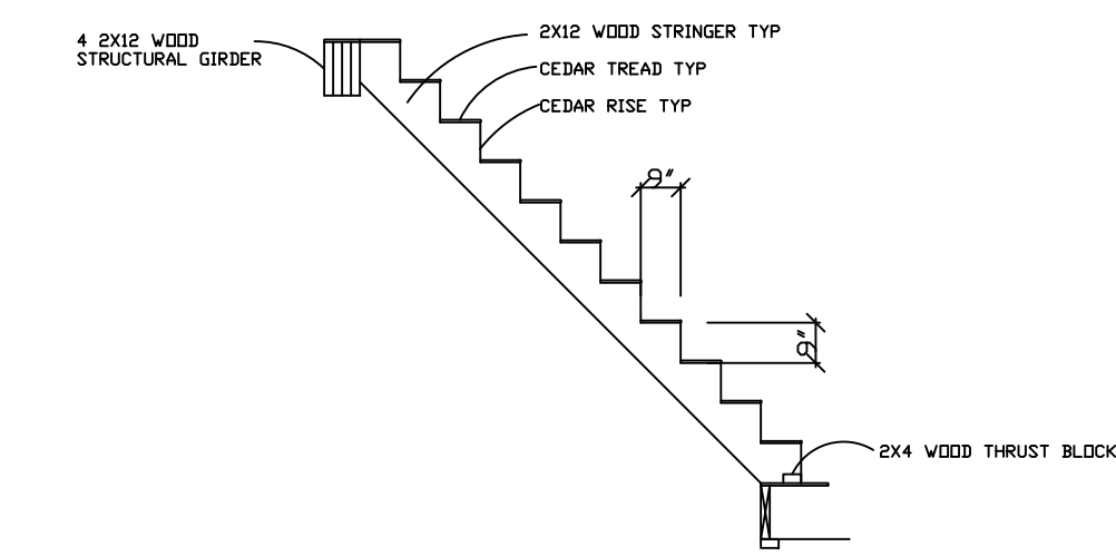
STAIR DETAIL Scale: 1/4"=1.0'
