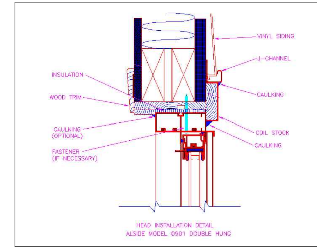
WINDOW DETAIL Scale: 1/4"=1.0'
