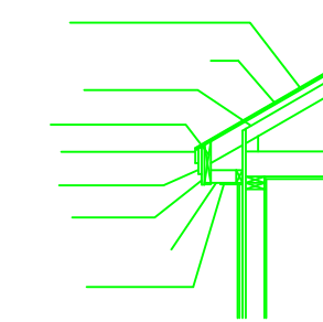
WALL DETAIL Scale: 1/4"=1.0'
