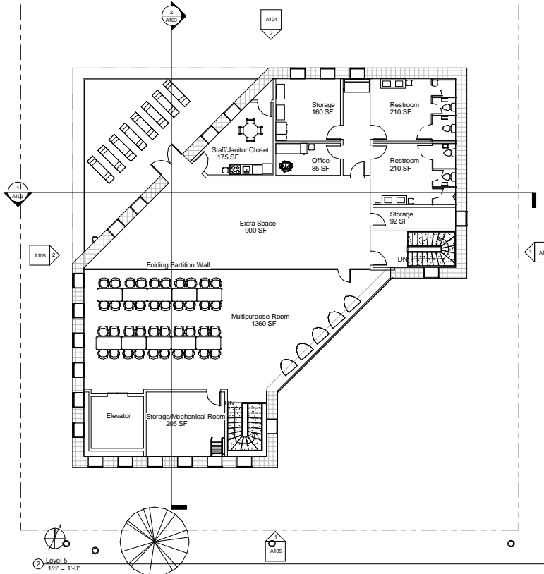
Level 5 1/8" = 1'-0"
