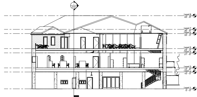
2 Section 2 1/8" = 1'-0"
